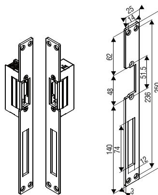
FP-GK250 Mortise mount
